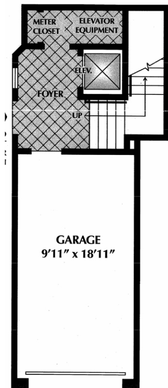
First Floor (9' Ceilings)
